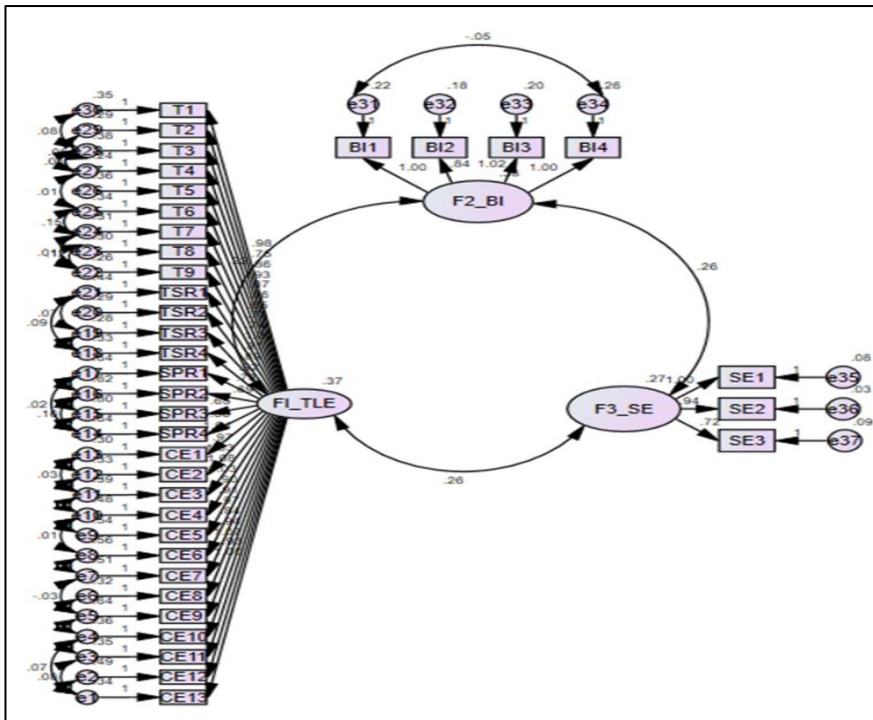
Figure 2: Confirmatory Factor Analysis Source: Covariance based structural equation modelling (2023)
